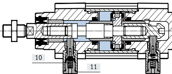
Standards-based cylinder
