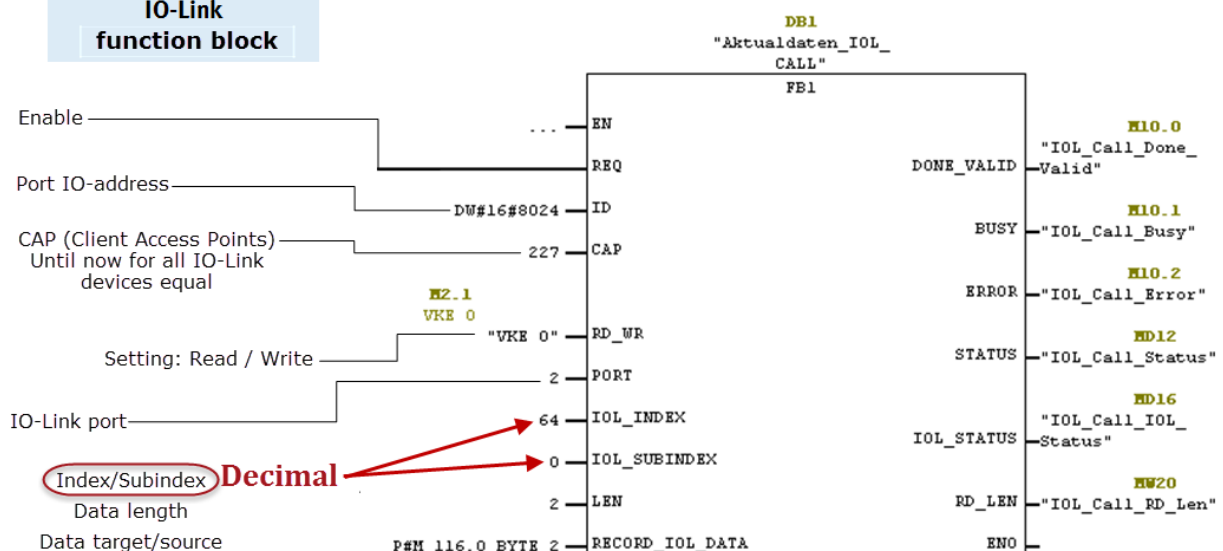
Figure 4.6. Fb1 description
