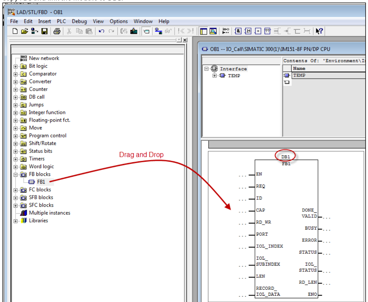
Figure 4.5. Creating Fb1
