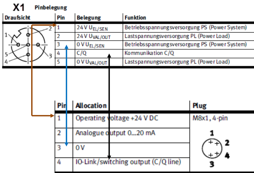
Figure 3.0: IO Link connection
