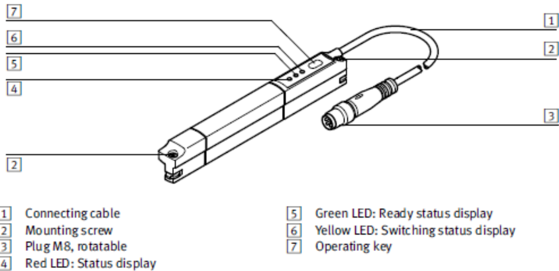
Fig. 1 Control sections and connections
