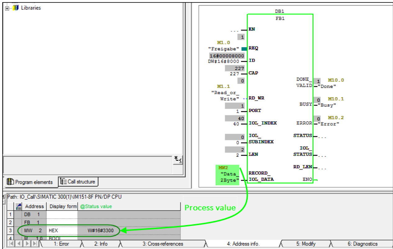
Figure 4.9. Online FB1
