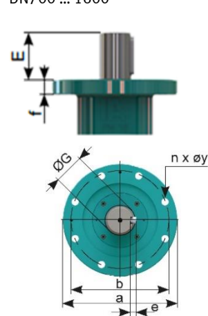
DN700 ... 1600
