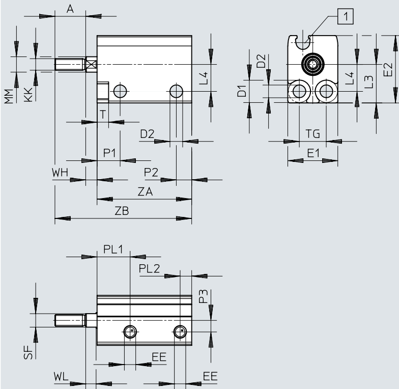
Dimensions – ADN-S-6 ... 10 – with male thread
