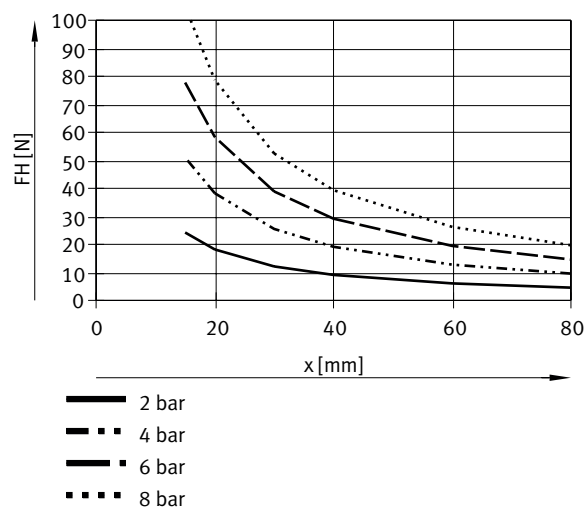
Gripping force FH per gripper jaw as a function of operating pressure and lever arm x – Internal gripping (opening), double-acting – DHRS-25
