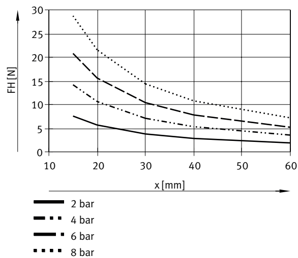
Gripping force FH per gripper jaw as a function of operating pressure and lever arm x – Internal gripping (opening), double-acting – DHRS-16
