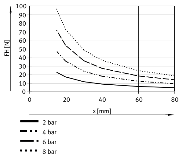
Gripping force FH per gripper jaw as a function of operating pressure and lever arm x – External gripping (closing), double-acting – DHRS-25
