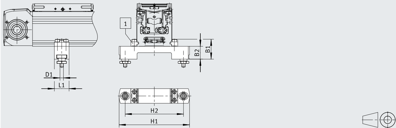
[1] Profile mounting
