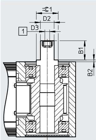
[1] Draw-off thread
