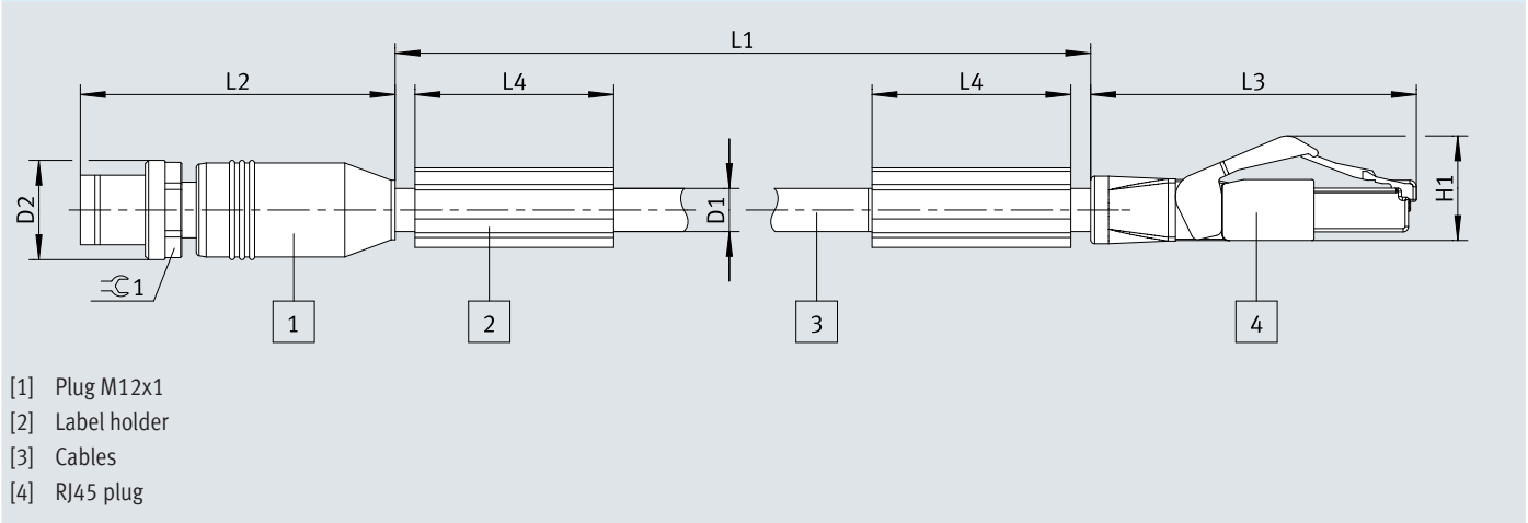
Dimensions – Plug M12 with plug RJ45, D-coded
