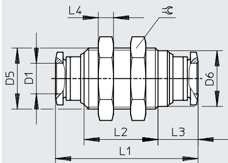
Dimensions – Push-in bulkhead connector QSS
