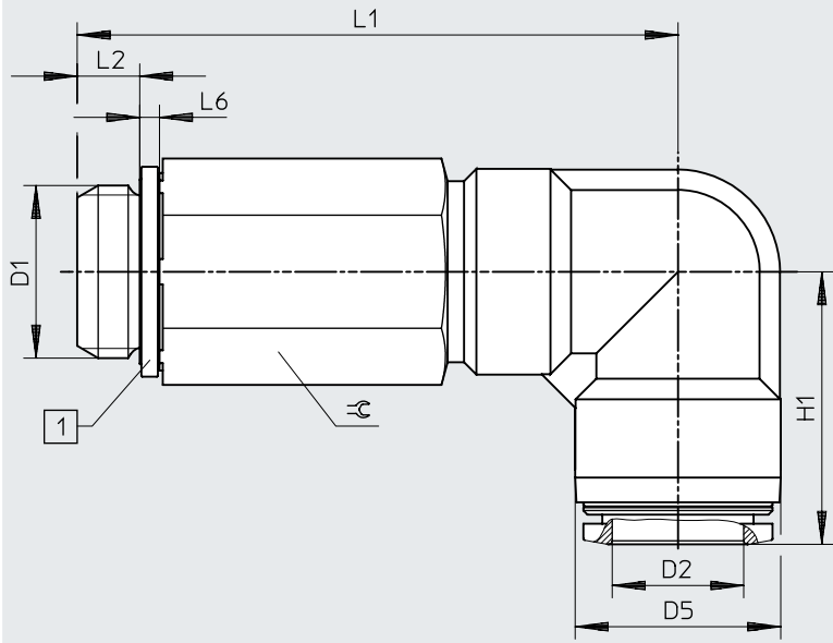
Dimensions – Push-in L-fitting, long QSL-...-16, G-thread with sealing ring Download CAD data www.festo.com
