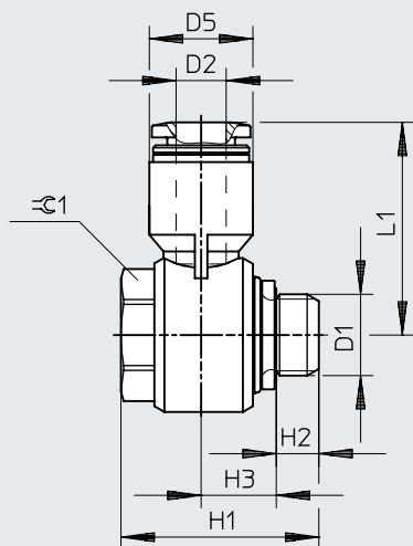
Dimensions – Push-in L-fitting QSLV, G thread with sealing ring
