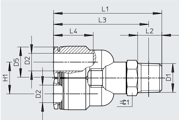
Dimensions – Push-in Y-connector QSY, R-thread Download CAD data www.festo.com
