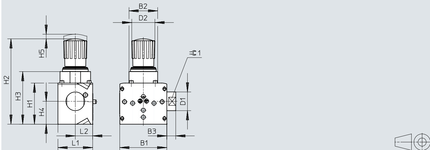
Dimensions – Filter regulator PCRI
