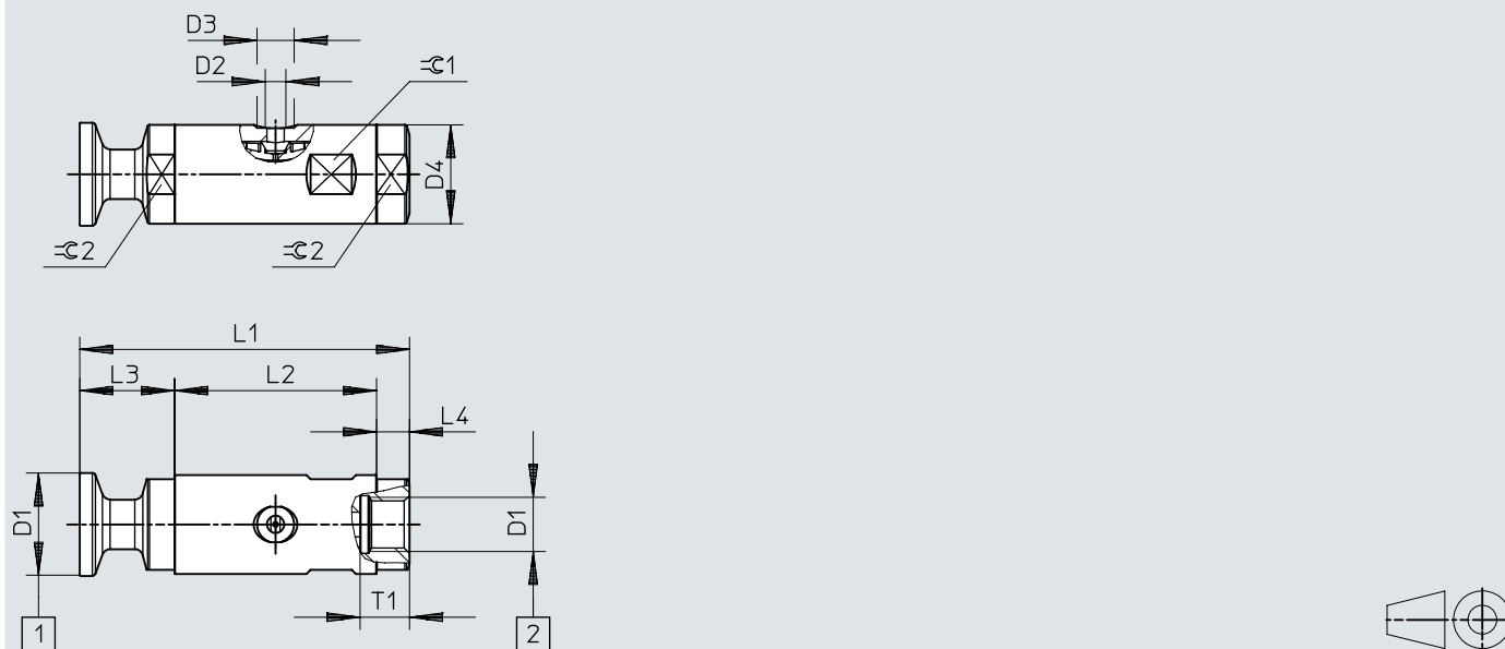
Dimensions – VZQA-...-M22U, nominal width 50 (part 2 of 2)
