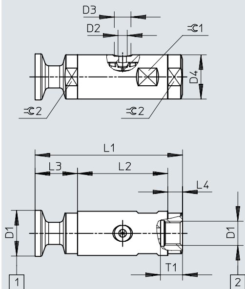
Dimensions – VZQA-...-M22U, nominal width 50 (part 1 of 2)
