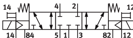
[5/3G] 5/3 directional control valve, mid-position closed
