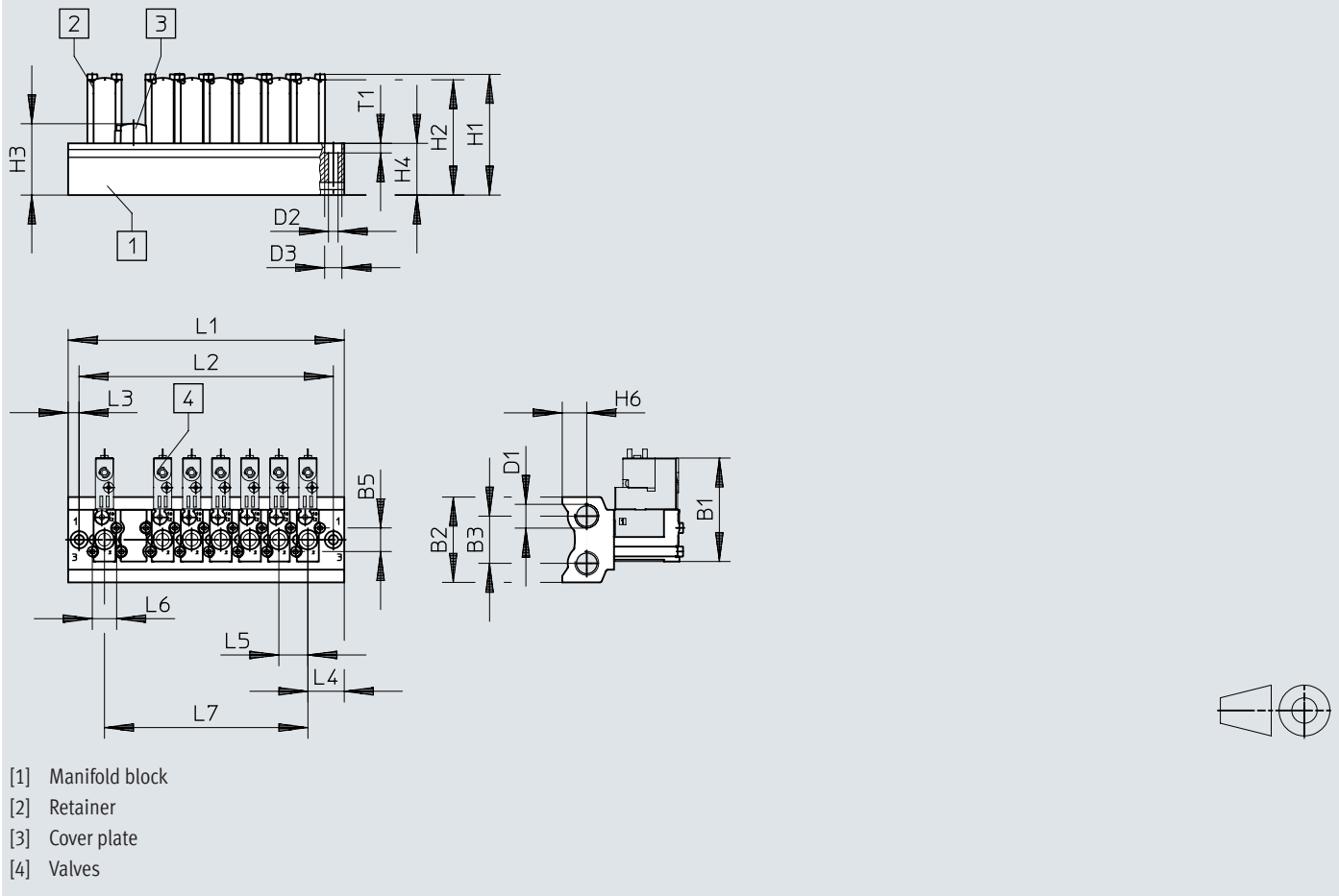
Dimensions – CPE10, connection block, fixed grid battery 3/2
