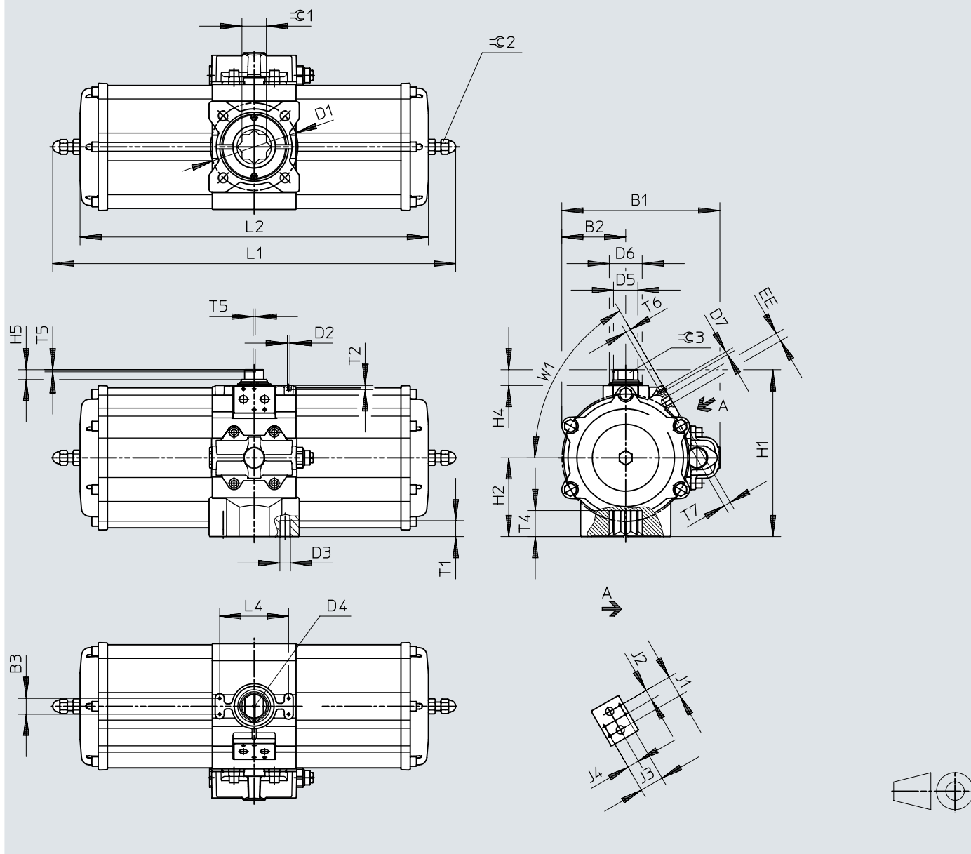
Dimensions – Size 1920, single-acting
