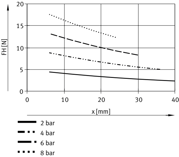
Gripping force FH per gripper jaw as a function of operating pressure and lever arm x – external gripping (closing), double-acting – DHPS-6
