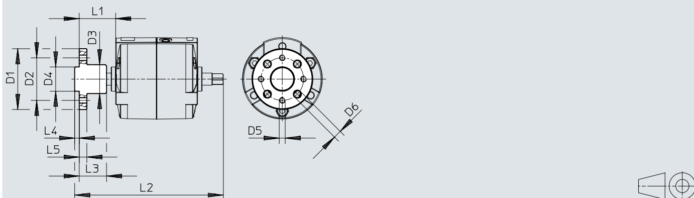
Dimensions – Push-on flange DARF for DRVS-12/16
