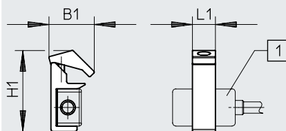
[1] Proximity switch SDBF
