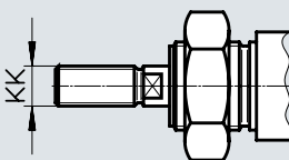
K5 – Special piston rod thread
