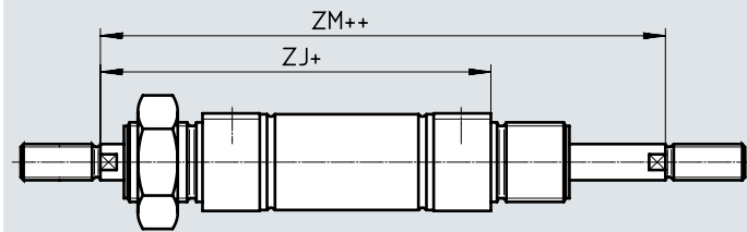
K2 – Extended male piston rod thread
