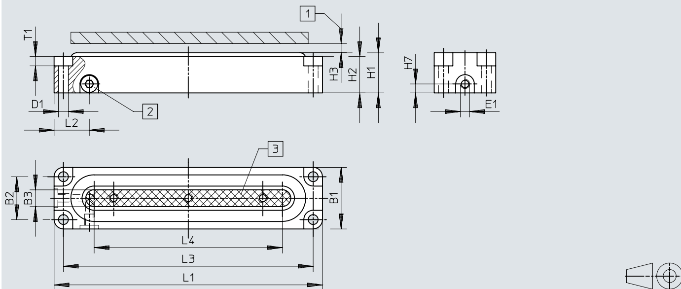
Dimensions – Clamping module, cuboid shape
