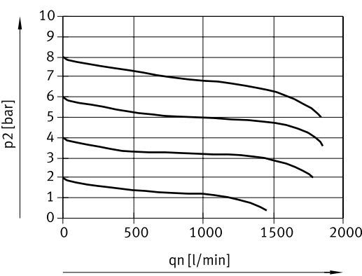
Standard flow rate qn as a function of output pressure p2 (FRC-1/4-D-MINI)
