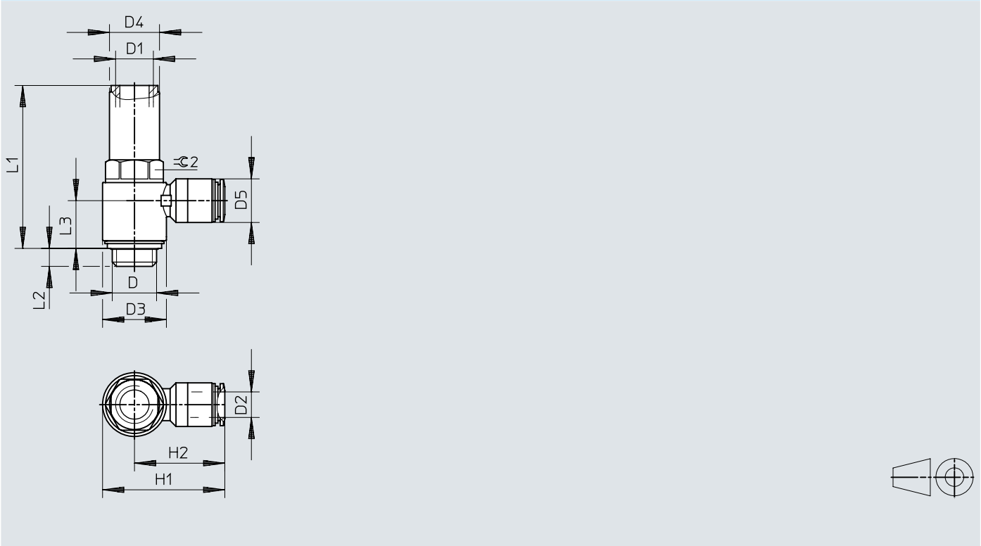
Dimensions – Plug connector HGL-1/2
