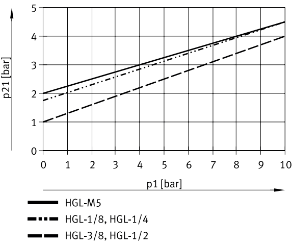
Minimum pilot pressure p21 as a function of operating pressure p1
