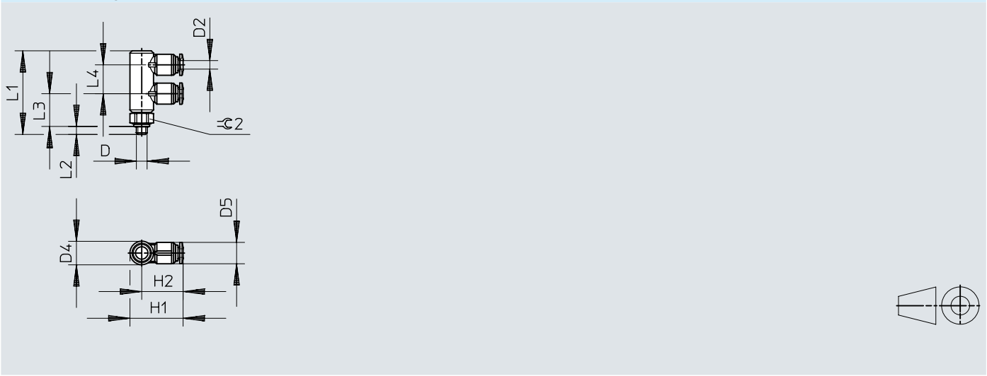
Dimensions – Plug connector HGL-M5
