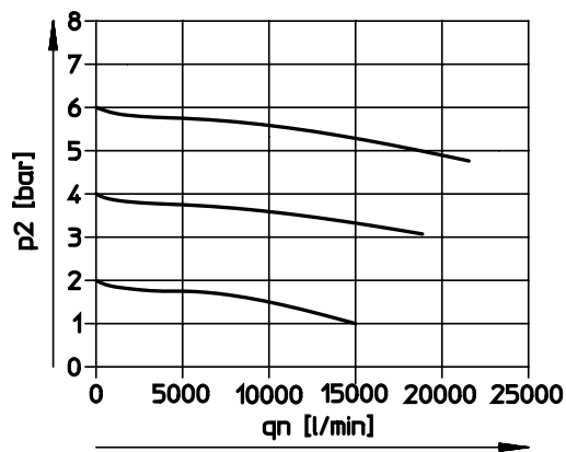
Pneumatic connection G1 1/2 with connecting plate MS12-AGH
