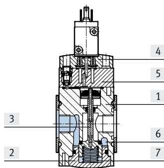
Soft-start valve
