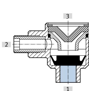
[SEU] Quick exhaust valve with silencer
