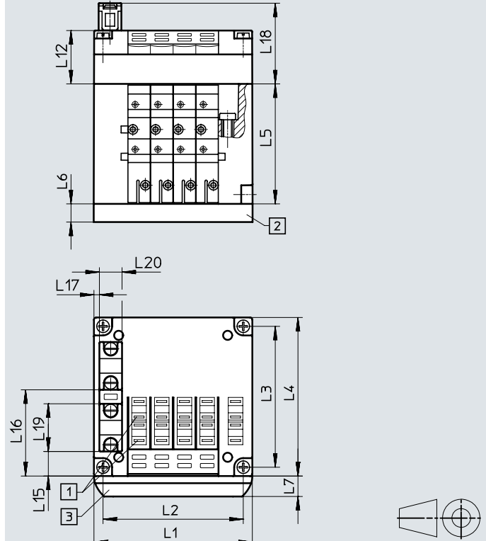
Valve terminal with AS-Interface connection – CPV10/14/18
