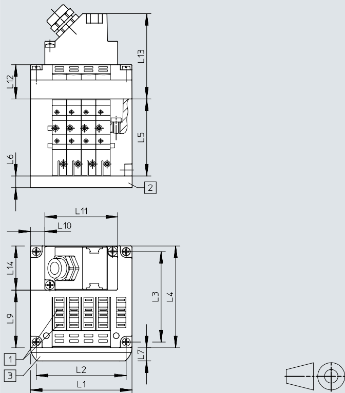
Valve terminal with multi-pin plug connection – CPV10/14/18
