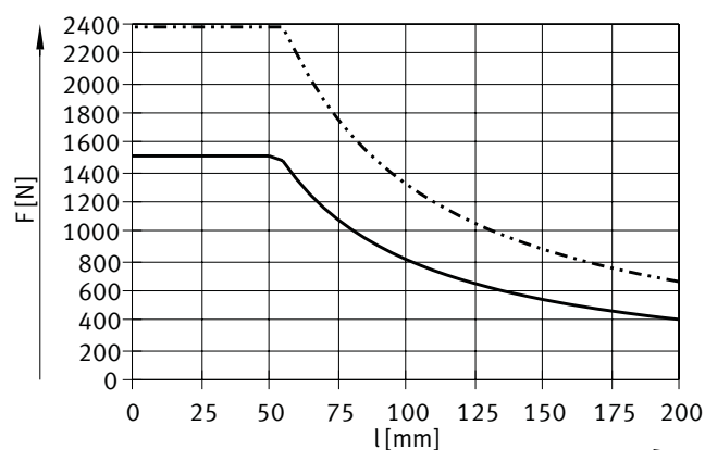
DFM-80 ... 100-GF, carrera de 80 ... 200 mm
