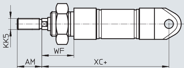
K5 – Special piston rod thread
