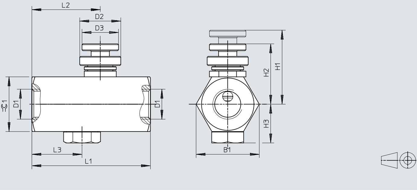
Dimensions – GRO-1/4
