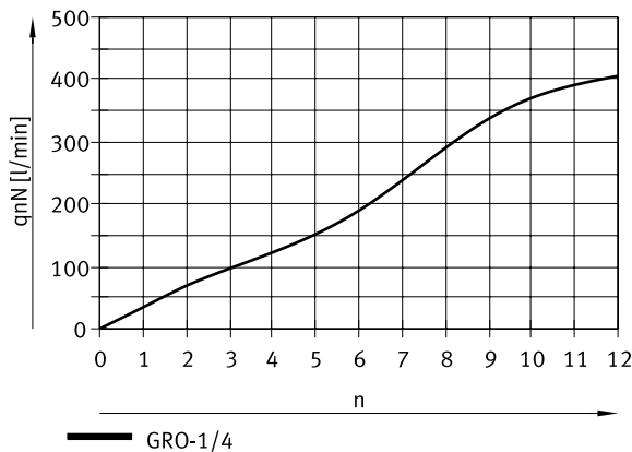
Standard nominal flow rate q_{nN} at 6 → 5 bar as a function of spindle rotations n (GRO-1/4)
