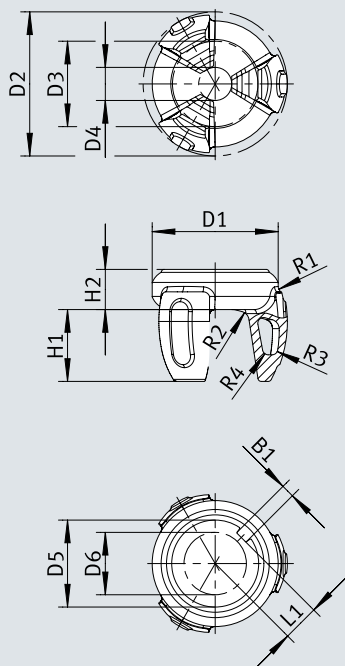
Dimensions – Gripper finger cap HAMA-GA-B33-40-3-S-40-BU
