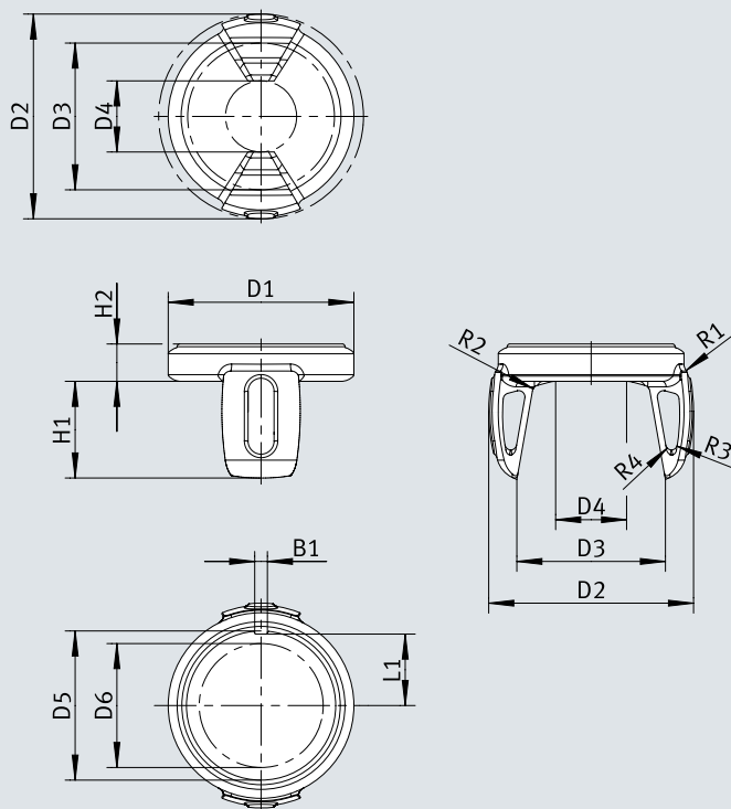
Dimensions – Gripper finger cap HAMA-GA-B33-70-2-S-40-BU
