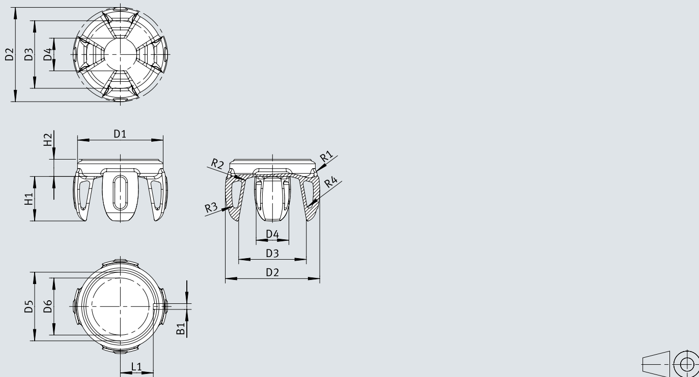
Dimensions – Gripper finger cap HAMA-GA-B33-70-4-S-40-BU
