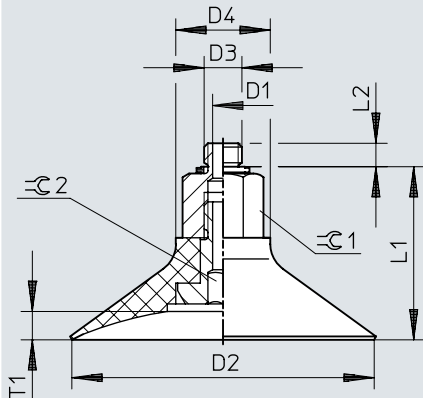
Dimensions – Suction cup with connector ESS-...-GT...
