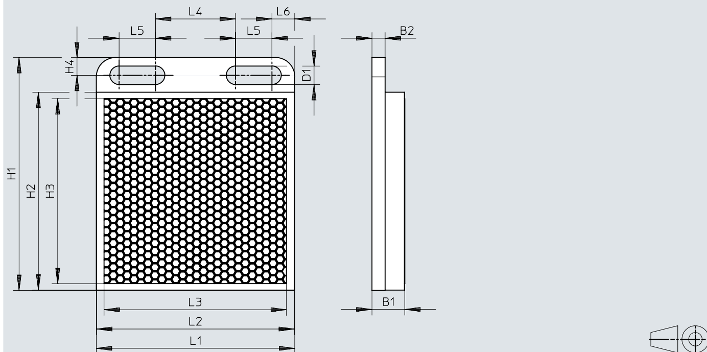
Dimensions – Reflector SARA-R-Q50
