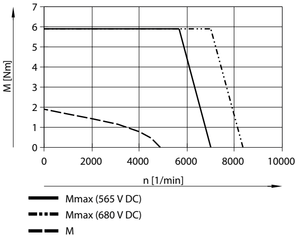
Torque M as a function of rotational speed n for EMMH-AS-68-HA-HS
