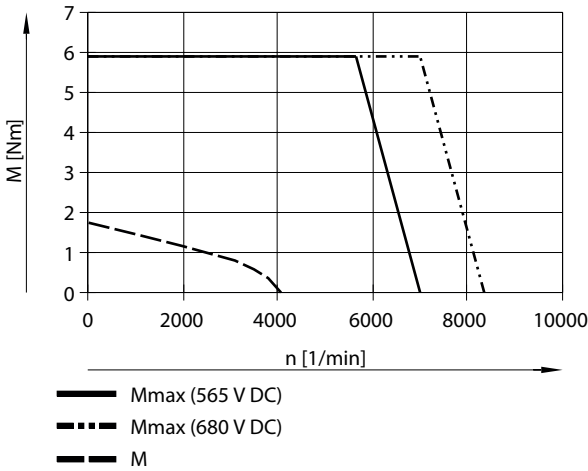
Torque M as a function of rotational speed n for EMMH-AS-68-HA-HS-B
