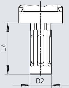
Dimensions – Silencer
