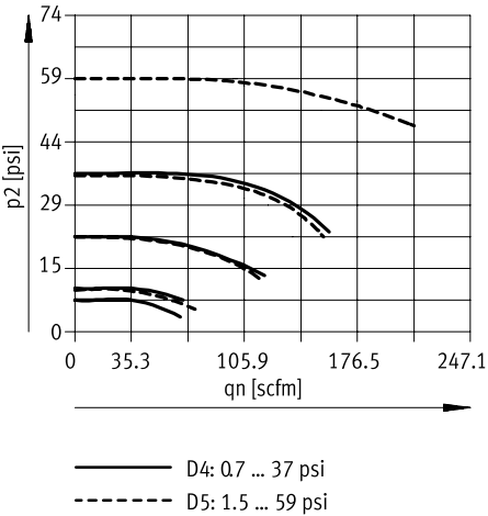
Normal flow rate q_n as a function of the outlet pressure p_2 ( p_1 = 147 psi) - MS6N-LRP-3/8
