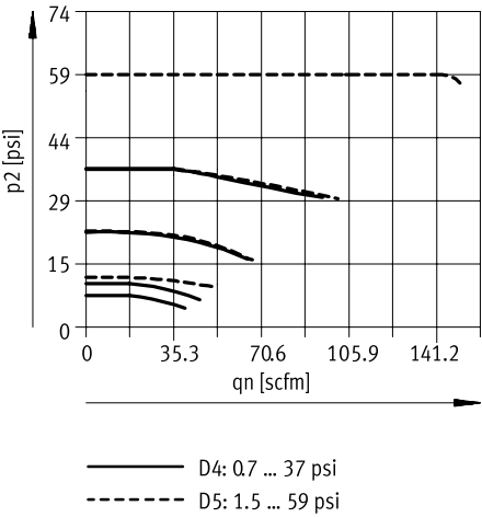
Normal flow rate q_n as a function of the outlet pressure p_2 ( p_1 = 147 psi) - MS6N-LRP-1/4
