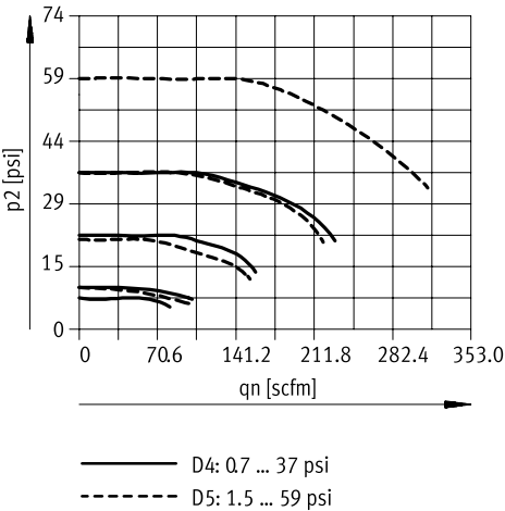
Normal flow rate q_n as a function of the outlet pressure p_2 ( p_1 = 147 psi) - MS6N-LRP-1/2
