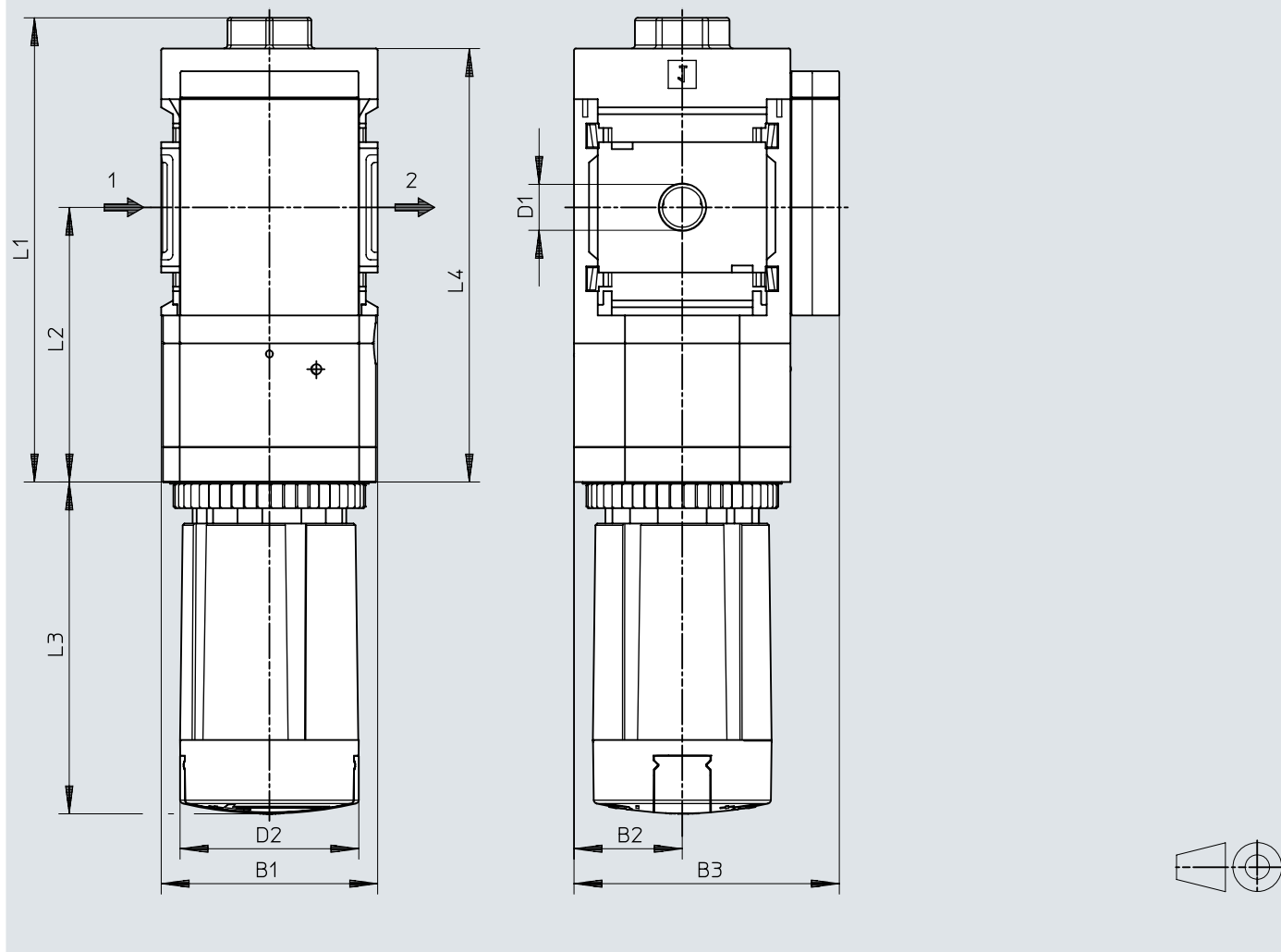
Dimensions – Alternative mounting position, rotary knob at the bottom
