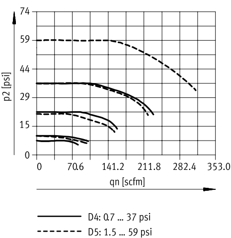
Standard flow rate qn as a function of output pressure p2 (p1 = 147 psi) – MS6N-LRP-1/2
