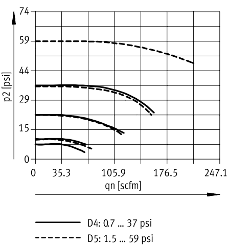
Standard flow rate qn as a function of output pressure p2 (p1 = 147 psi) – MS6N-LRP-3/8
