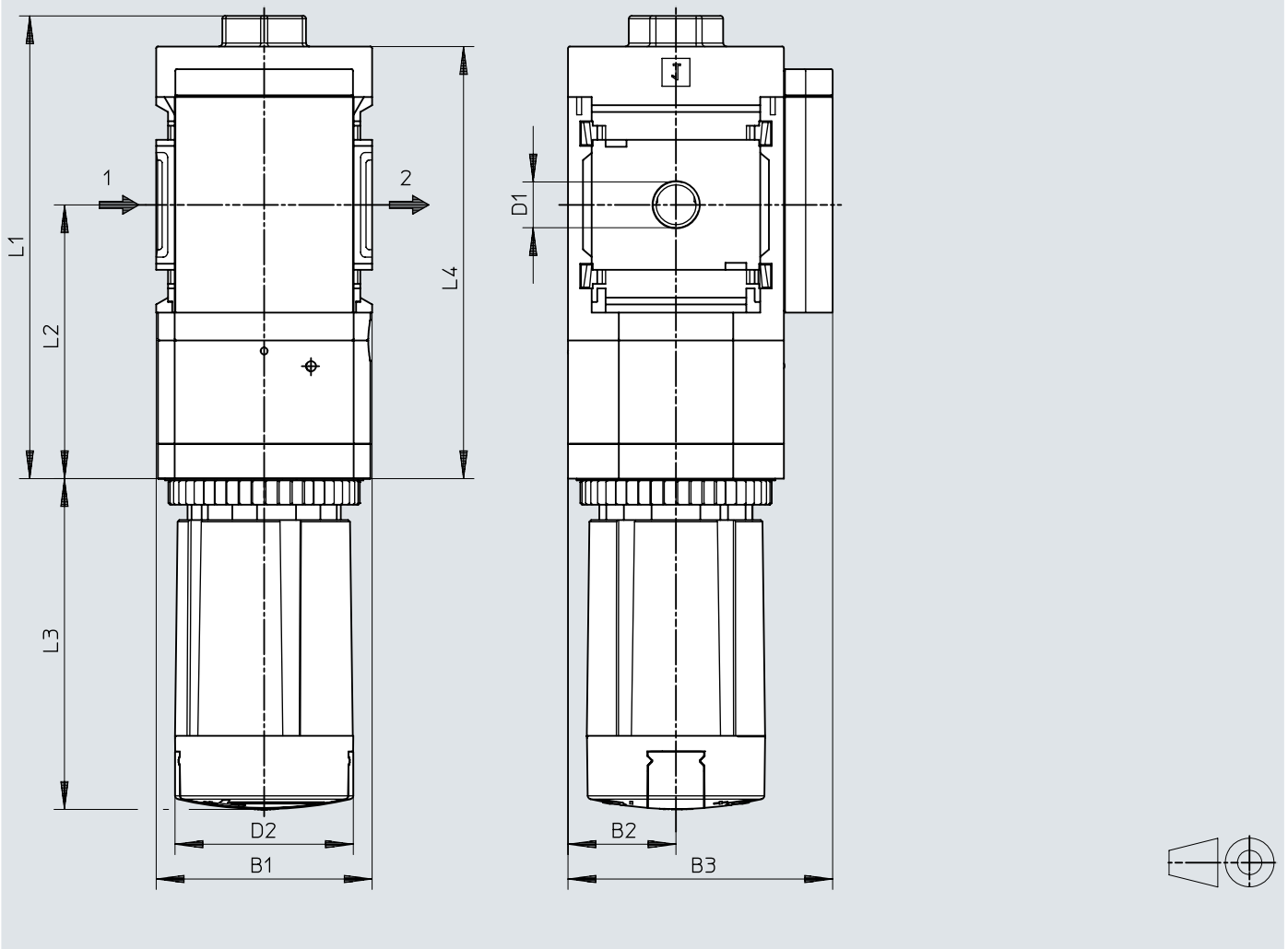
Dimensions – Alternative mounting position, rotary knob underneath
