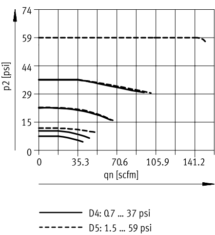
Standard flow rate qn as a function of output pressure p2 (p1 = 147 psi) – MS6N-LRP-1/4
