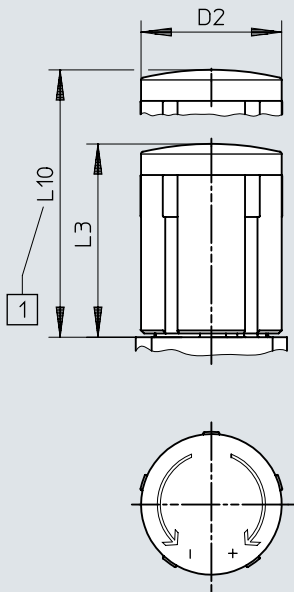
Dimensions – Rotary knob, long, with latch
