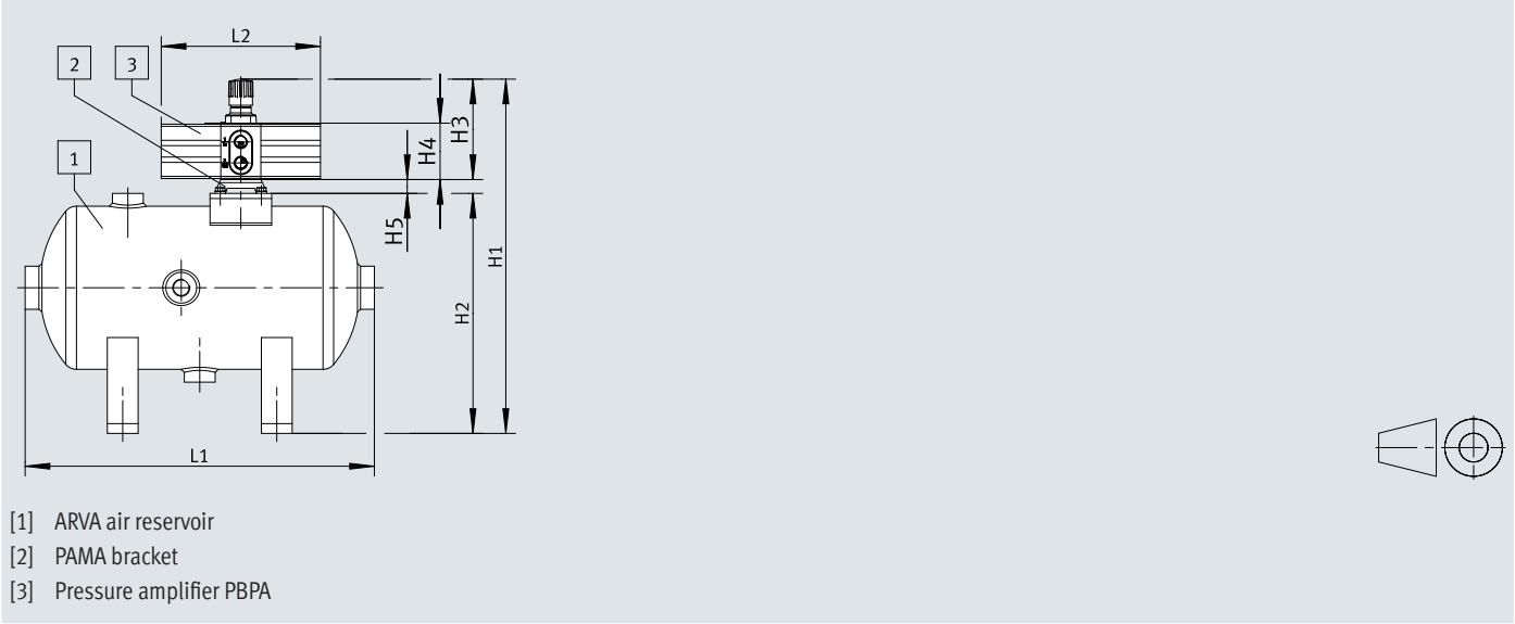
Dimensions – ARVA-...-P1 with PBPA pressure amplifier
