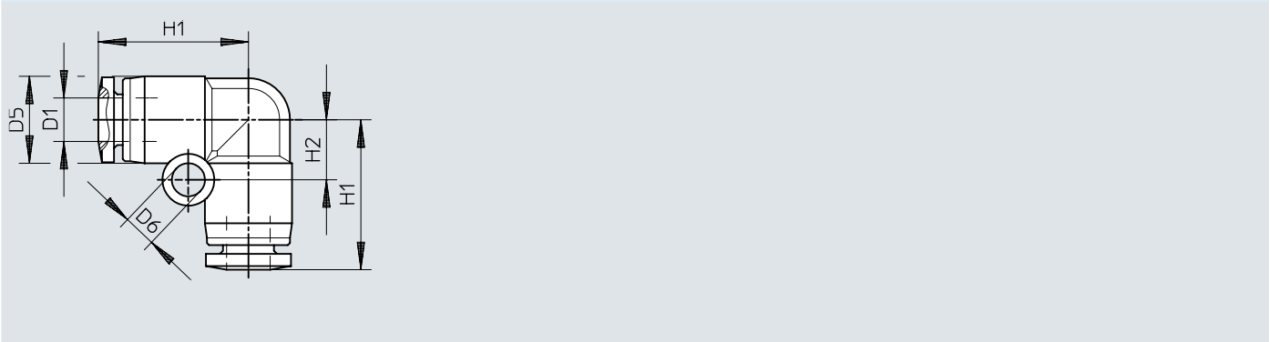
Dimensions – Coude union QBML-...T
