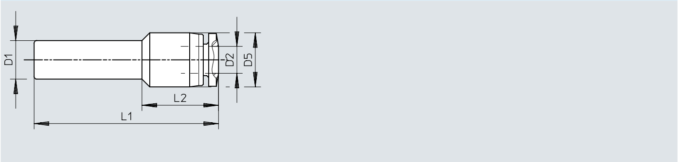
Dimensions – Union QBM-...H
