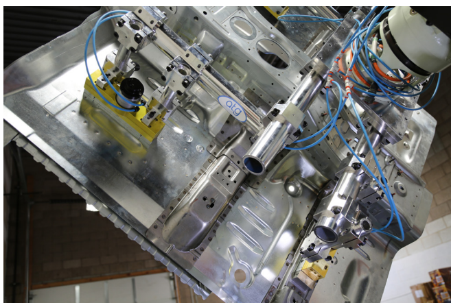
Floor Pan End of Arm Tooling (EOAT)
