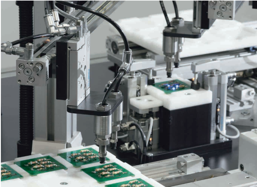
Figure 7: Precise placement using mini-slides
