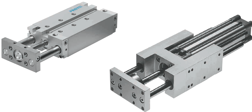
Figure 1. A guided drive like the Festo DFM (left) includes integrated guide rods and requires no assembly while a guide unit like Festo's FENG plus a standard cylinder (right) requires assembly.
