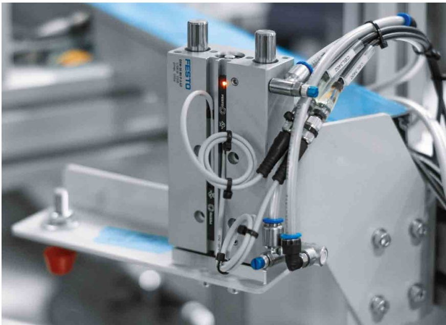
Figure 9: The DFM base model series is Festo's most popular pneumatic guided drive.
