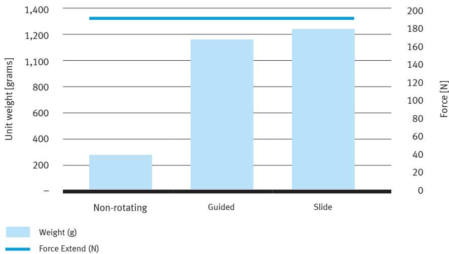
Figure 5: Weight to linear force comparison.
