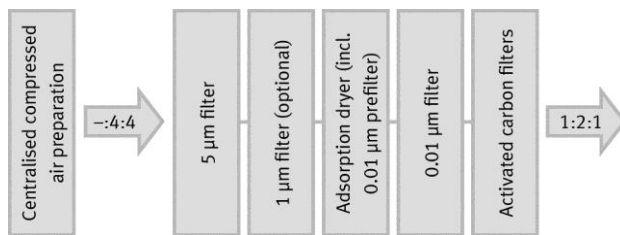
Filter cascade for compliance with class 1:2:1
