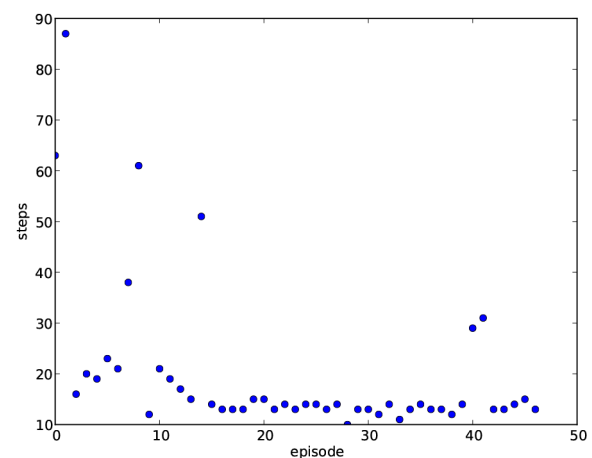
Fig. 7 Learning high-level manipulation for a given goal orientation. The blue dots represent the required number of high-level actions to achieve the goal orientation. Outliers are due to the sphere being dropped during manipulation. After about 15 episodes a robust strategy has been found.
