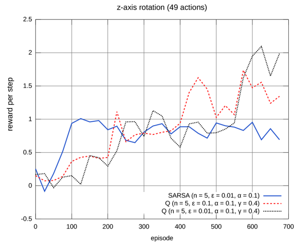
Fig. 5 Learning high-level action (discrete state space). The reward per step shows the amount of rotation a single action has performed in the goal direction. The curves show single execution of different discrete learning agents with different learning parameters.
