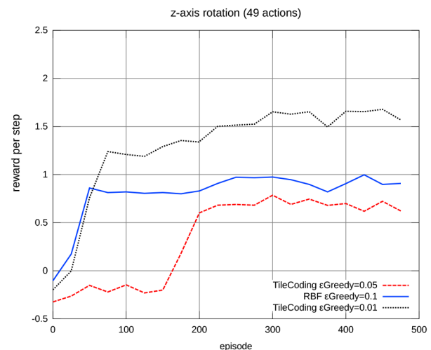
Fig. 6 Learning high-level action (continuous state space). The reward per steps shows the amount of rotation a single action has performed in the goal direction. The curves show different continuous learning agent with different learning parameters.
