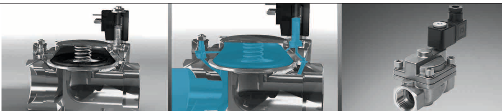
Servo-controlled...
