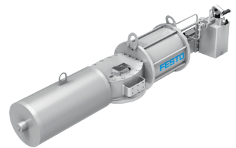
Single-acting with hydraulic manual override
