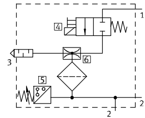
Circuit diagram 2
