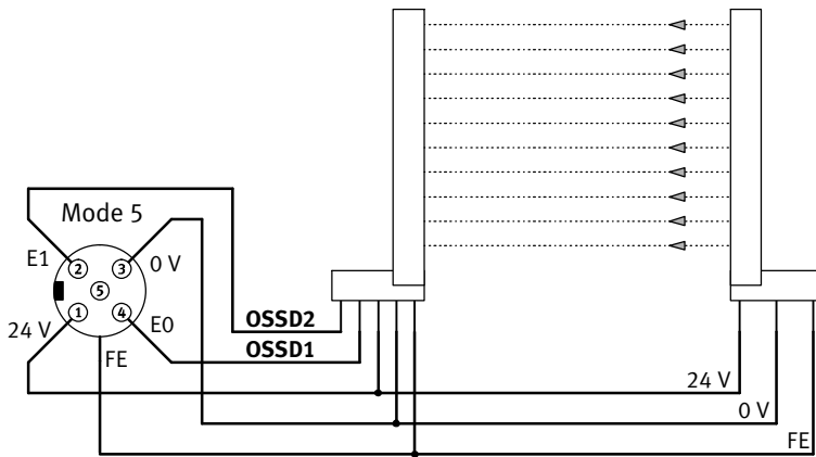
Fig. 1/7: Connection of a light grid
