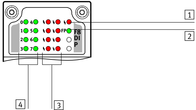
Fig. 4/1: LED display of input module CPX-F8DE-P
