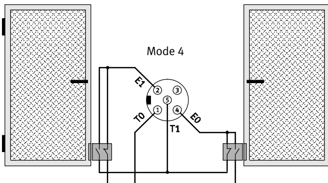
Fig. 1/9: 2 protective door sensors on one channel pair
