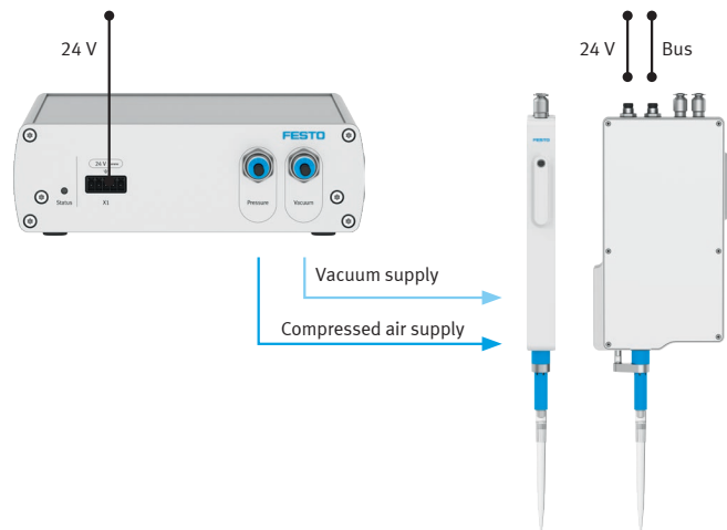
Pressure and vacuum generator PGVA-2
