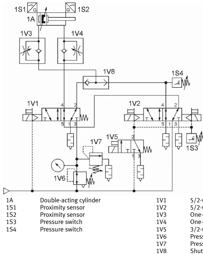
Figure 12: Actuating a drive with a monostable 5/2-way valve and a bistable valve with the additional requirements: extension with reduced pressure and protection against unexpected start-up
