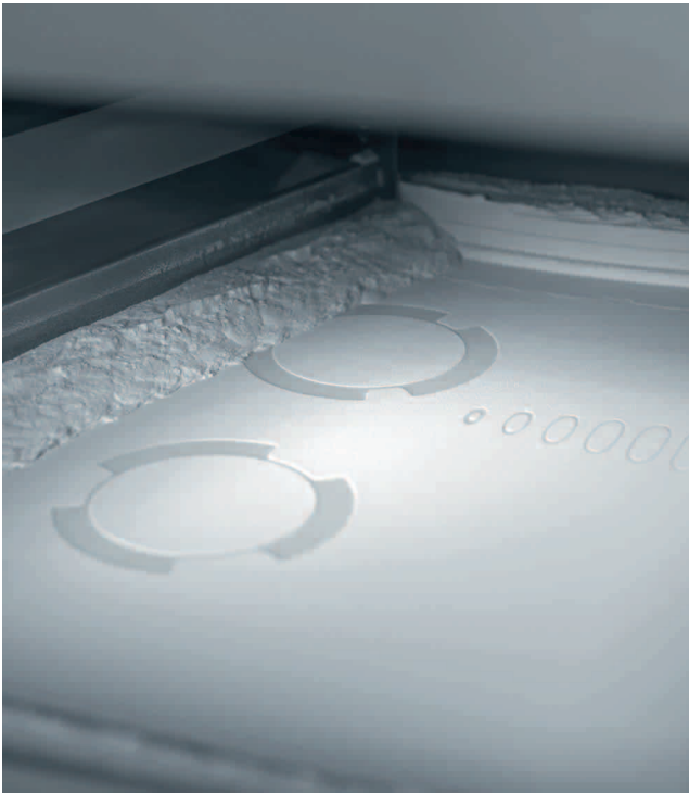
A flexible polyamide structure from additive manufacturing
