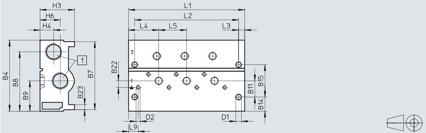
[1] Port 1 and 3: G3/8
