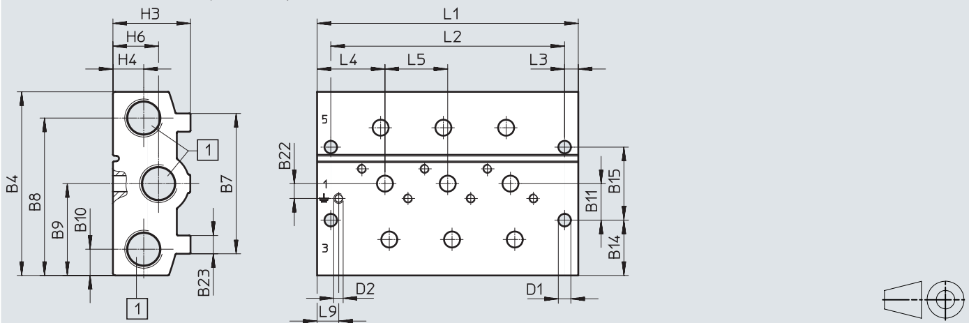
[1] Port 1, 3 and 5: G3/8
