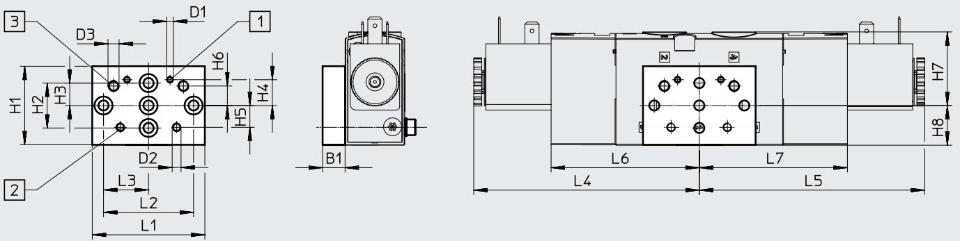
[1] Mounting hole for size 25
