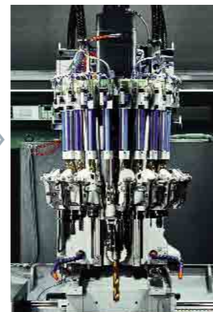
Integration cylinder for fast tool changing
